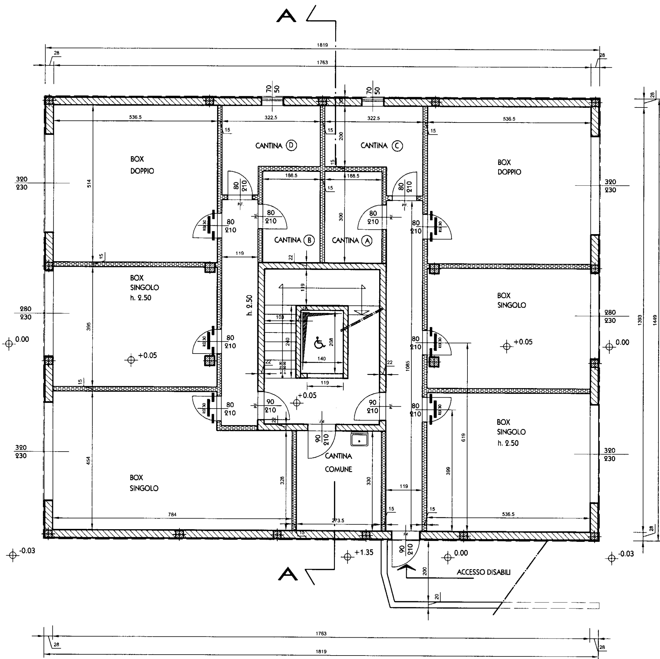
PIANO SEMINTERRATO
